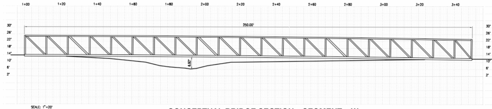
CONCEPTUAL BRIDGE SECTION – SEGMENT 5 W 250' LENGTH - 10' HEIGHT
