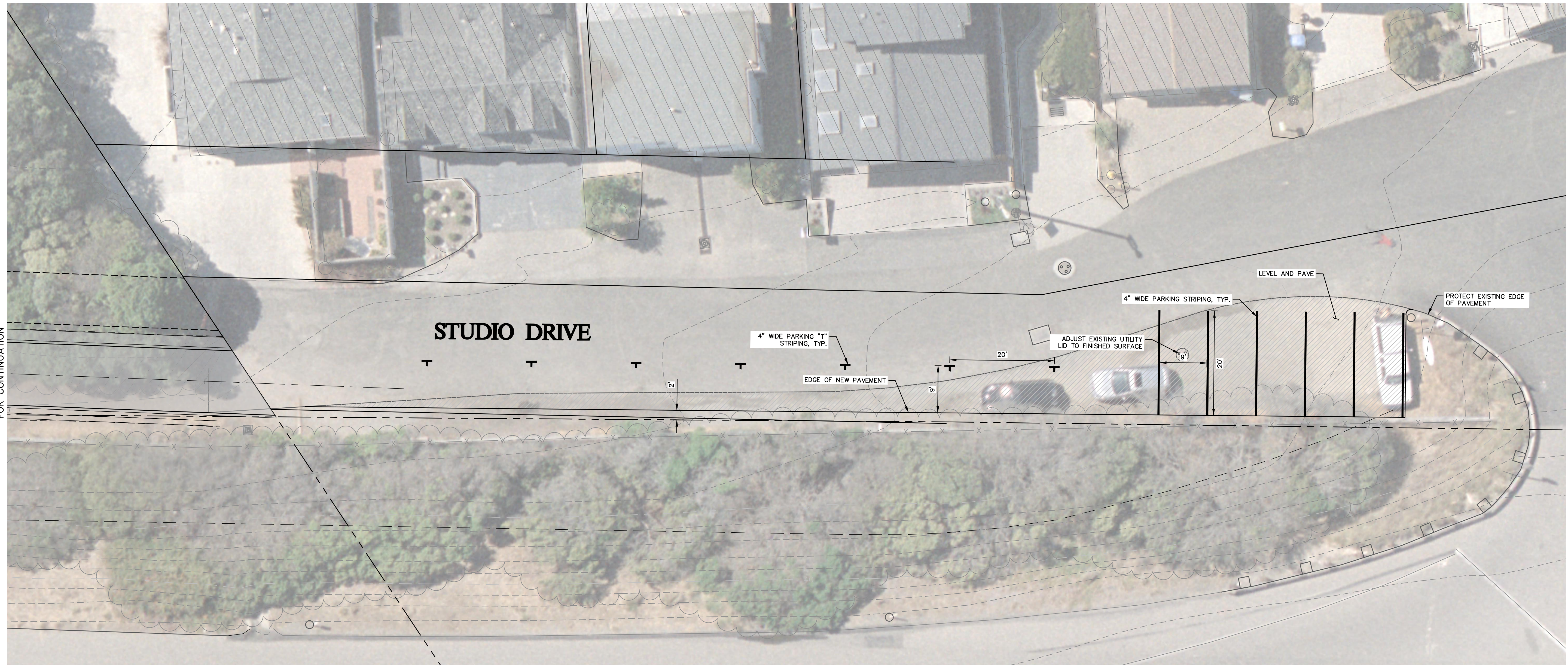
STUDIO DRIVE PARKING IMPROVEMENT PLAN
