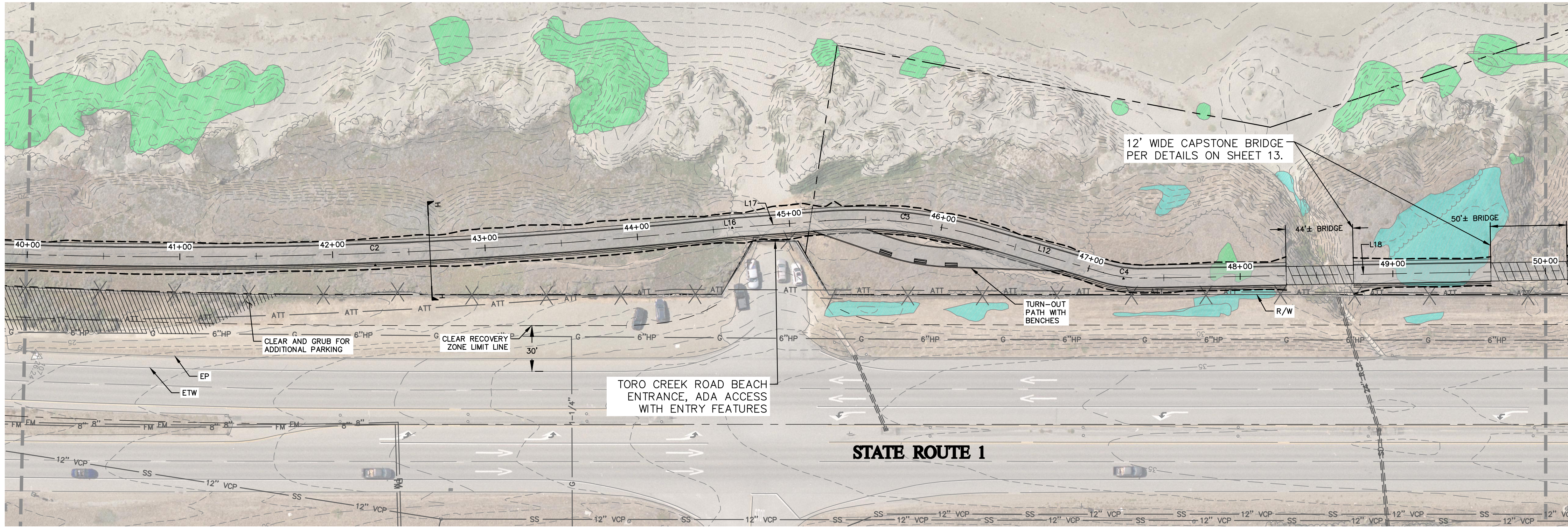
CLASS 1 PATHWAY – PLAN VIEW
