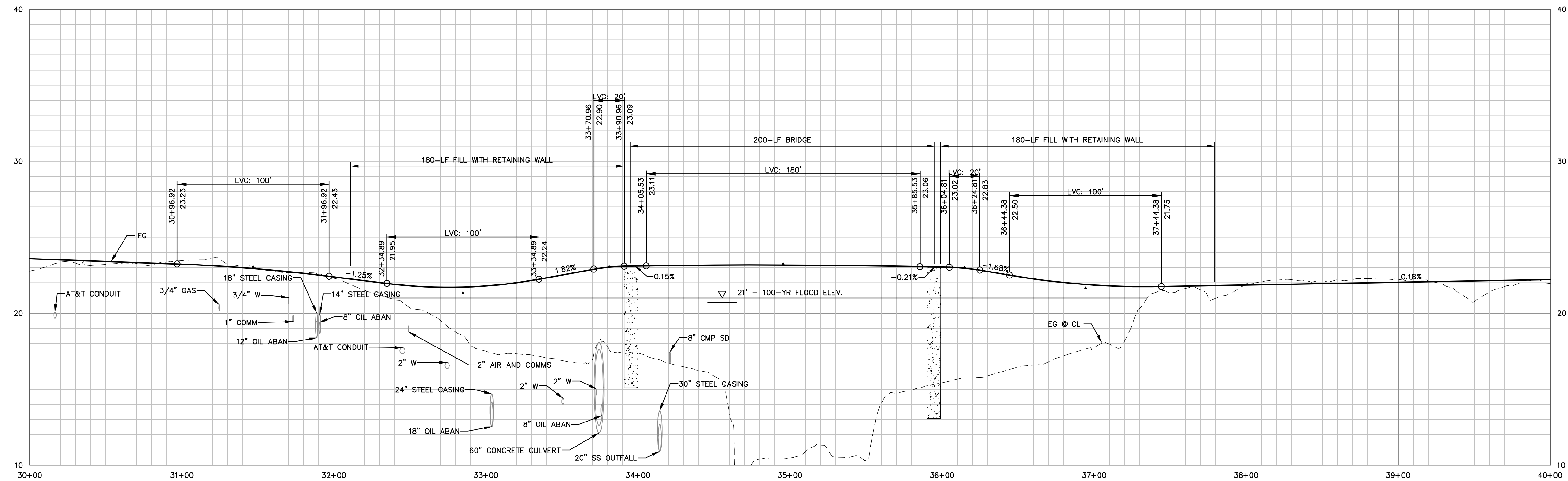
CLASS 1 PATHWAY - PROFILE VIEW SCALE: HORIZ 1"=40'; VERT 1"=4'
